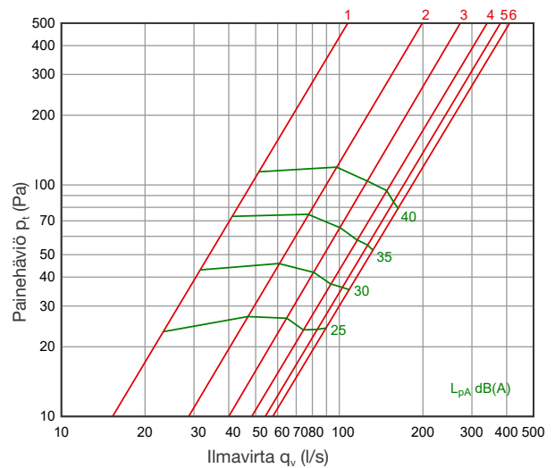
DEP 250 + SKDM 200/250
