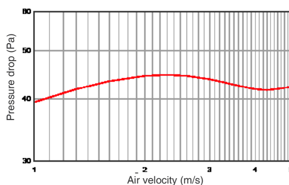
RVKS pressure drop in vertical duct
