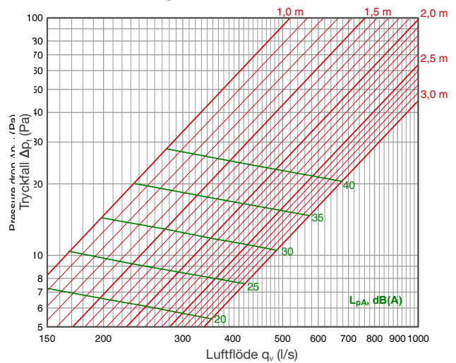
Tilluft: Perforeringsmönster SPx3
