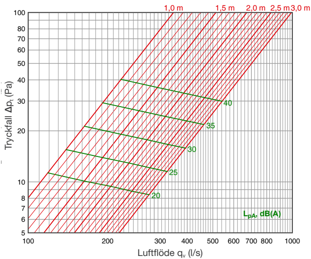
Tilluft: Perforeringsmönster SPx2
