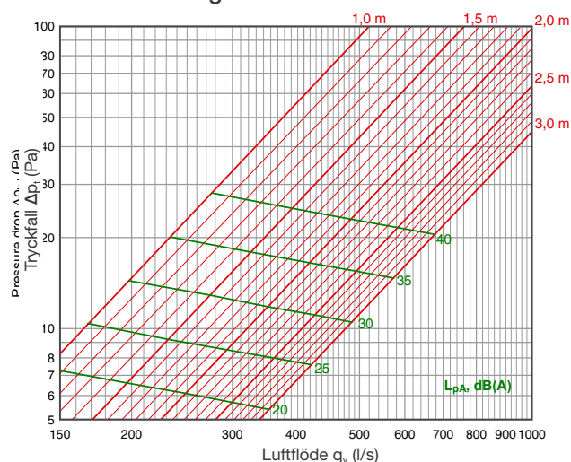
Tilluft: Perforeringsmönster SP×3
