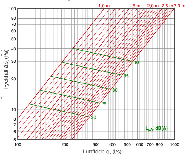
Tilluft: Perforeringsmönster SP×2
