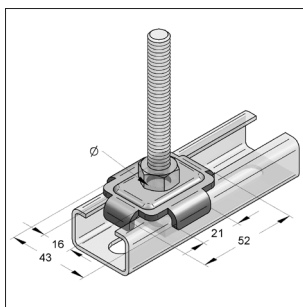
Profile holder combi
