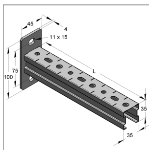
STEX console 35/35 Profile opening on bottom side
