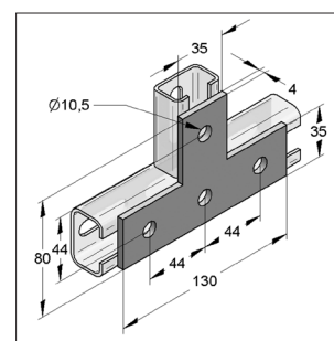
Flat connector 35/4 T-shape
