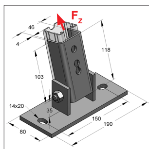
Joint holder with base plate horizontal
