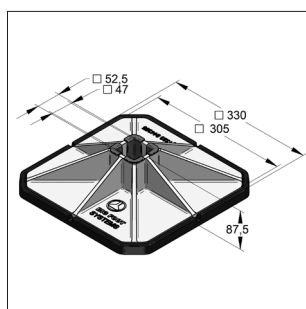
Rooftop holder Big Foot® 305 mm complete
