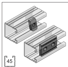
Threaded-/ tooth plates page 27
