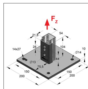
Holder square for C-profile rail
