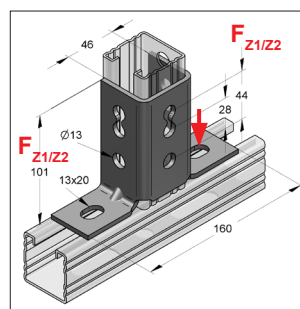
Angle connector C 45 180°
