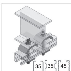
Girder connection horizontal page 59
