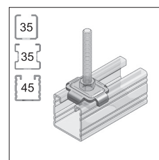
Profile holder page 39
