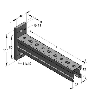
STEX console 35/42 Profile opening on bottom side
