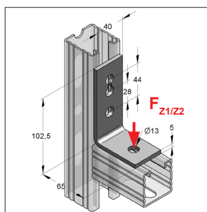
3-hole angle 40/5 L
