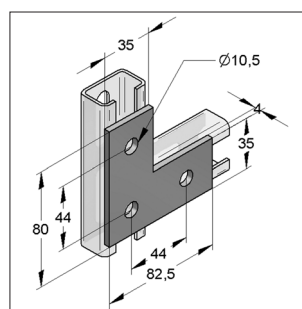
Flat connector 35/4 L-shape
