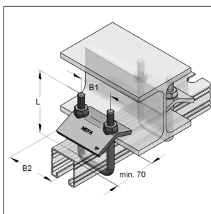
Clamping bow M10 45/60
