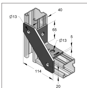
Universal knot K
