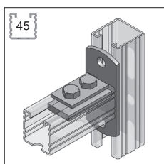
Front Connector page 37
