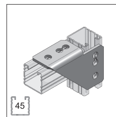
Corner angle page 36
