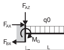
Loading condition 3 (LC3)
