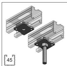
STEX 45 GP and GB page 23
