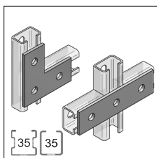
Flat connector page 16
