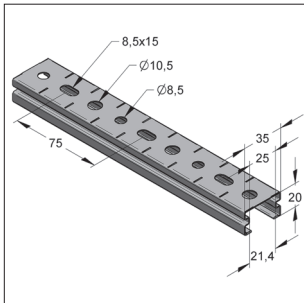
STEX profile rail 35/20
