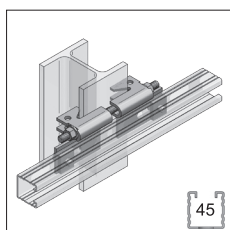
Girder connection vertical page 58
