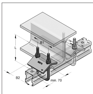
Clamping bow M8 35
