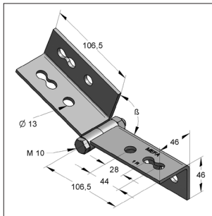
Profile joint connector
