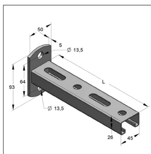
Console C 45/26/1,5 mm Profile slot at bottom side
