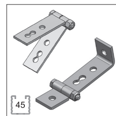
Joint connector page 43
