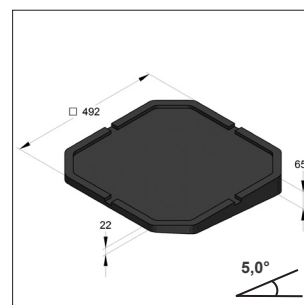
Rubber wedge 450 mm 5,0°
