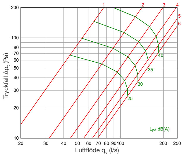
DEK 250 + SKDM 200/250
