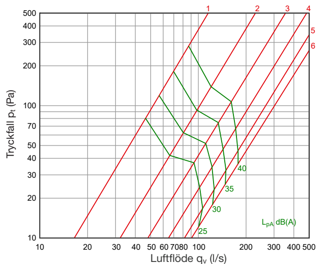
DEP 250 + SKDM 200/250
