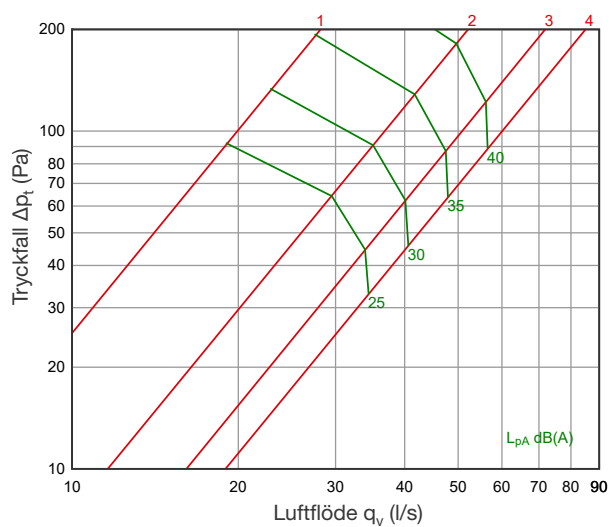
DEK 125 + SKDM 100/125
