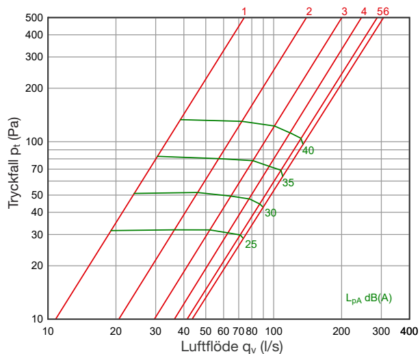
DEP 200 + SKDM 160/200
