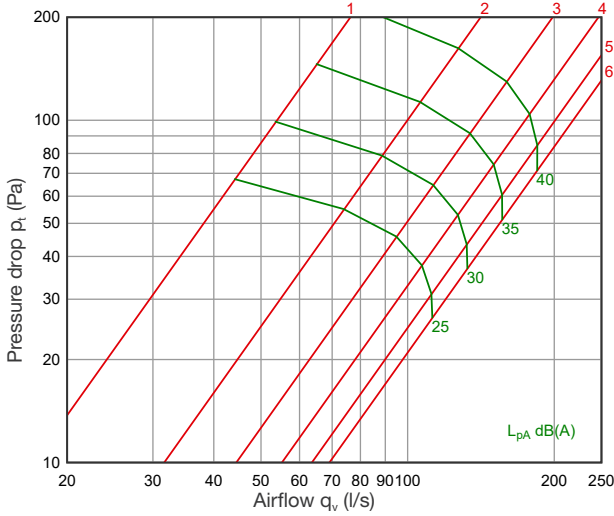
DEK 250 + SKDM 200/250
