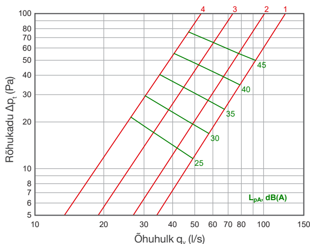
MRO 200×150
