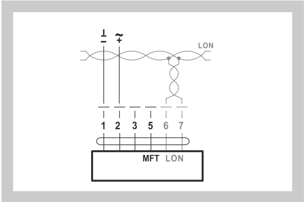
Fig. 12 Wiring of actuators LMV-D3-LON and NMV-D3-LON
