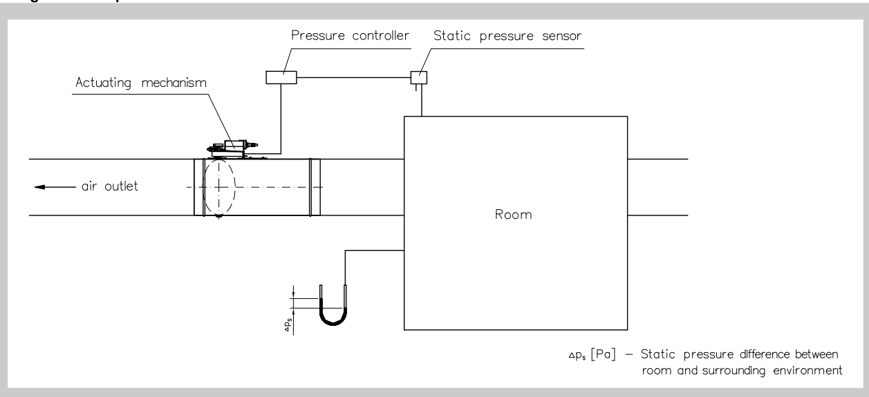
Fig. 4 Room pressure control
