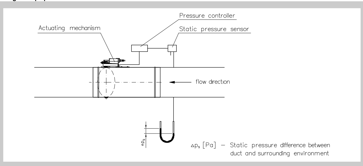
Fig. 3 Pipe pressure control
