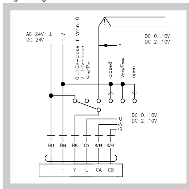
Fig. 20 Regulator 227VM-024-...-MB and 227PM-024-...-MB
