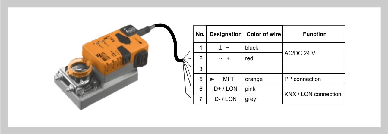
Fig. 10 Actuators LMV-D3-KNX, NMV-D3-KNX, LMV-D3-LON and NMV-D3-LON
