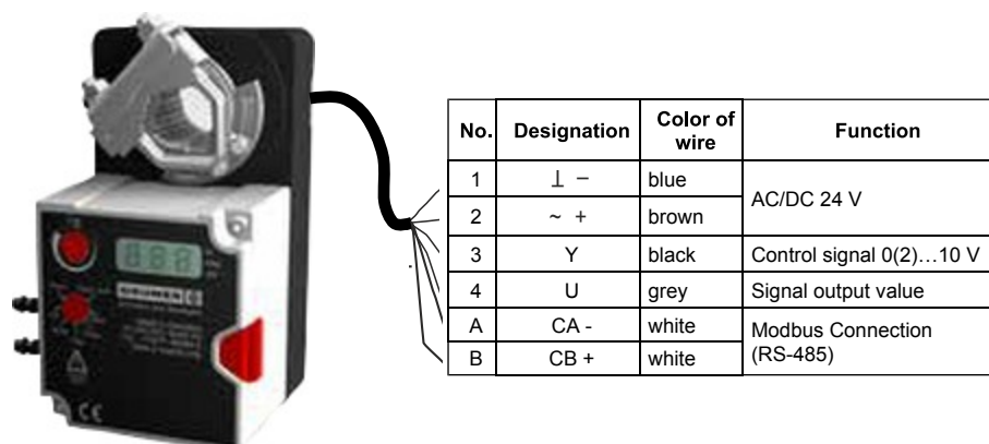
Fig. 18 Regulators 227VM-024-... -MB and 227PM-024-... -MB
