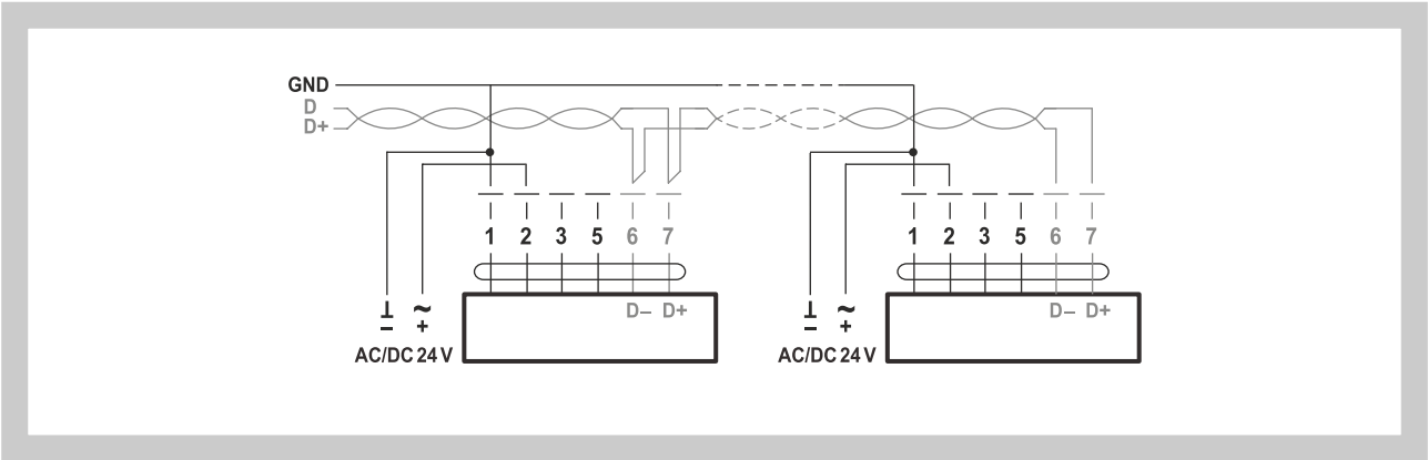
Fig. 9 Wiring of LMV-D3-MOD, NMV-D3-MOD and SMV-D3-MOD on the serial line RS-485
