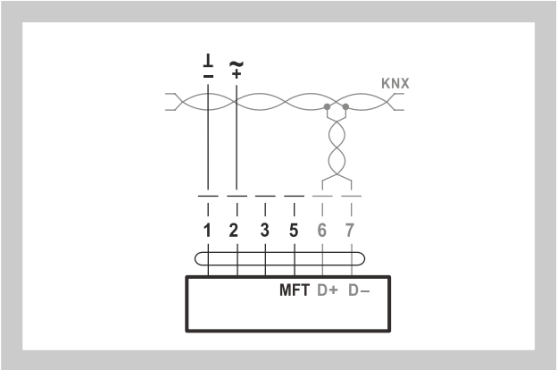
Fig. 11 Wiring of actuators LMV-D3-KNX and NMV-D3-KNX
