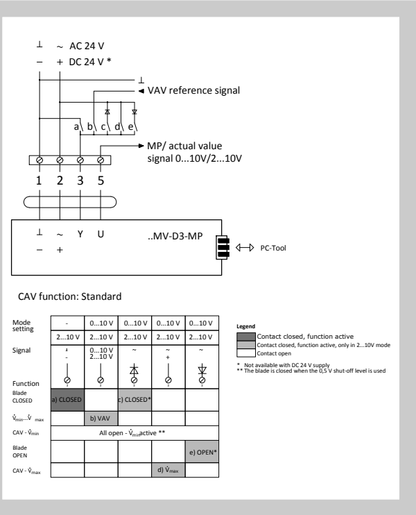
Fig. 6 Air flow control with LMV-D3-MP, NMV-D3-MP and SMV-D3-MP
