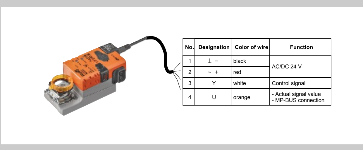
Fig. 5 Regulator LMV-D3-MP, NMV-D3-MP and SMV-D3-MP
