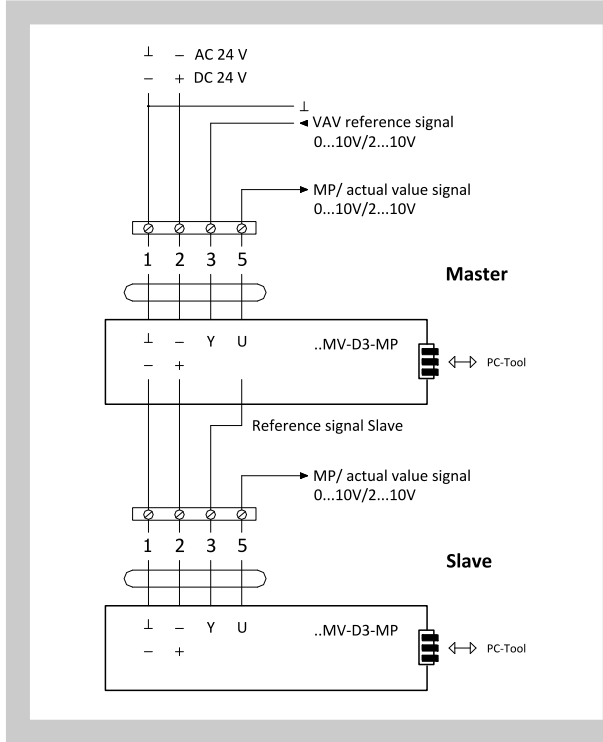
Fig. 7 Master-slave flow control with actuators LMV-D3-MP, NMV-D3-MP and SMV-D3-MP
