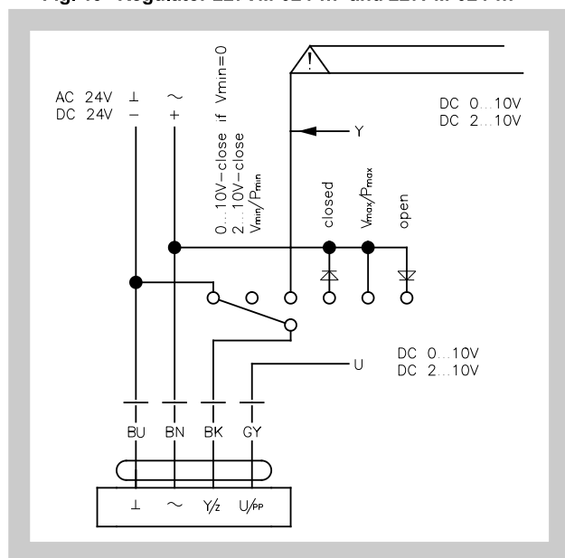
Fig. 19 Regulator 227VM-024-... and 227PM-024-...
