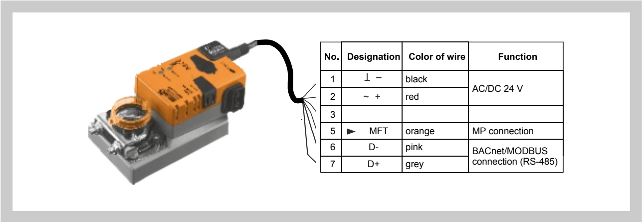
Fig. 8 Actuators LMV-D3-MOD, NMV-D3-MOD and SMV-D3-MOD
